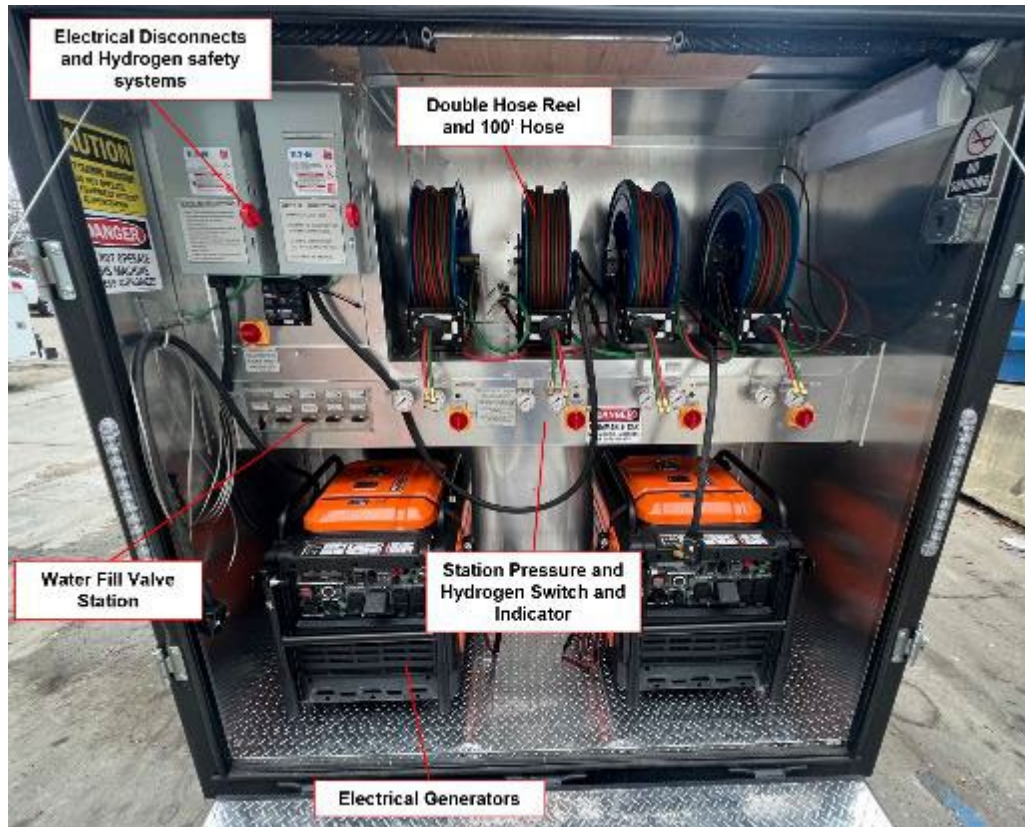
Trailer Rear Overview
