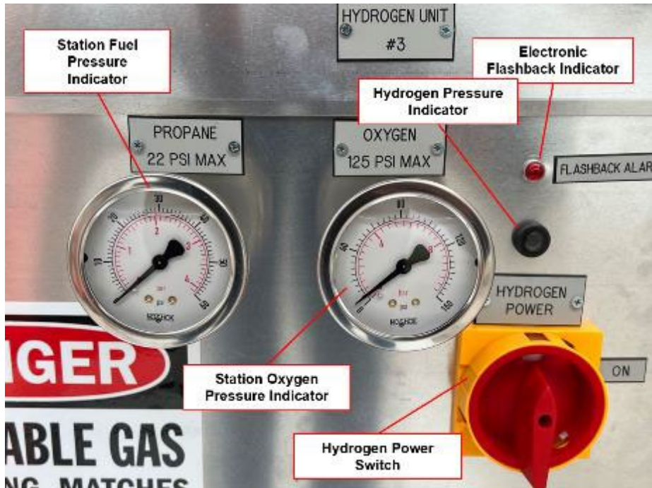
Station Pressure Indication and Hydrogen Control (Trailer Rear)
